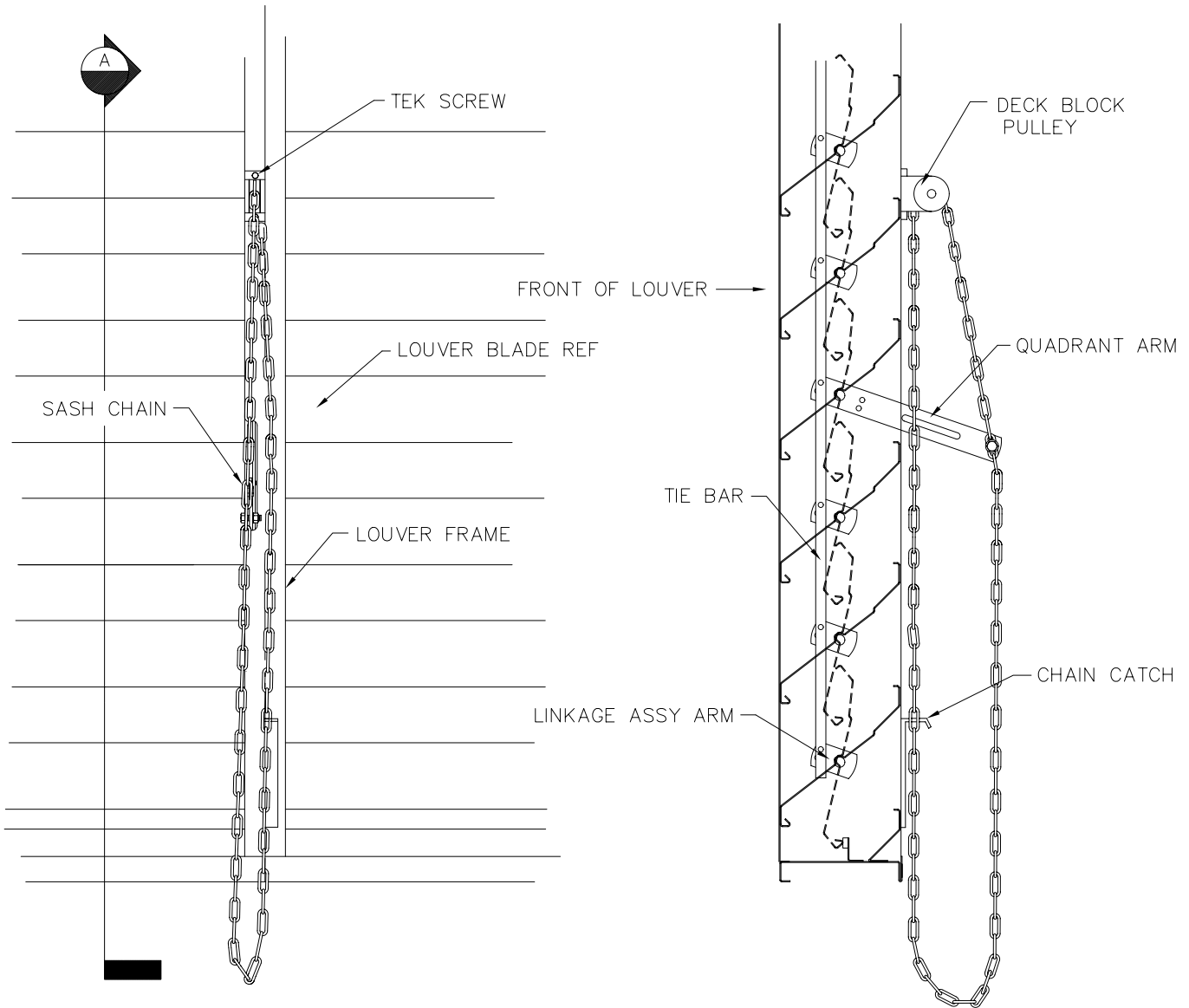
PARTIAL REAR ELEVATION N.T.S. ELEVATION
